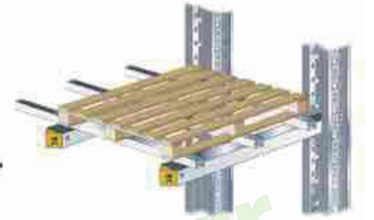
6 Travesaño / Cross member / Traverse
