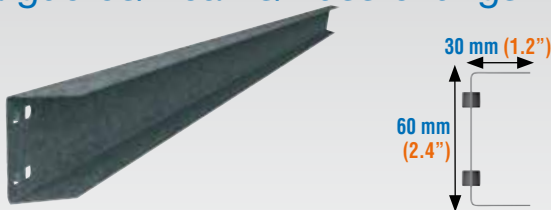
Larguero Serie U122 - Beam U122 Series
