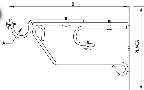
Soporte Techo Extensible (para Barra de 16, 19 y 25) - Extending Ceiling Support
