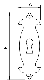
Escudo Bocallave - Plate With Keyhole
