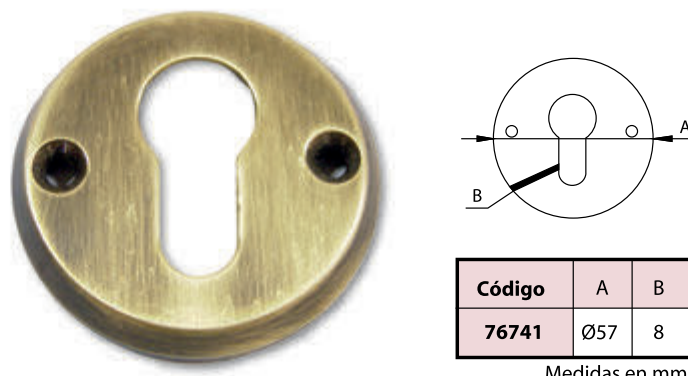
Placa Bocallave Latón Patinado - Patinated Brass Keyhole Plate
