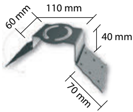
Cod.- 11112 - (110x60 mm.) Soporte Abatible Weather Vane Support
