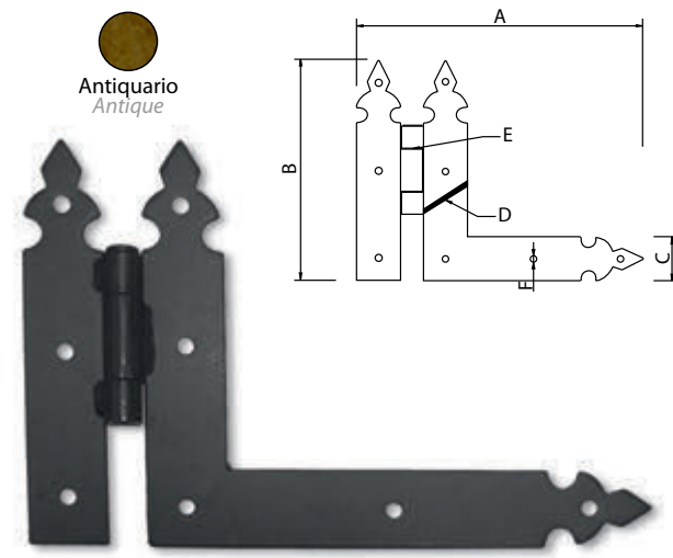
Bisagra "L" (derecha o izquierda) - Wrought Hinge (right-left)
