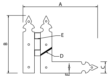
Bisagra "L" (derecha o izquierda) - Wrought Hinge (right-left)
