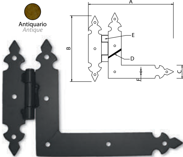
Bisagra "L" (derecha o izquierda) - Wrought Hinge (right-left)
